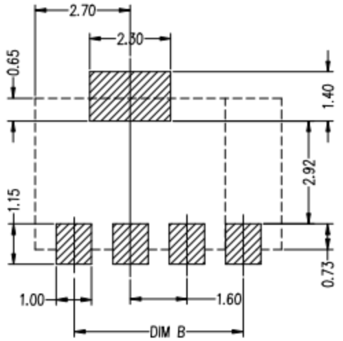
3&4PIN LAYOUT RECOMMENDED PCB LAYOUT TOL:(±0.05)
