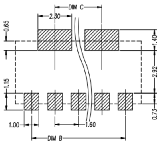
3&4PIN LAYOUT RECOMMENDED PCB LAYOUT TOL:(±0.05)
